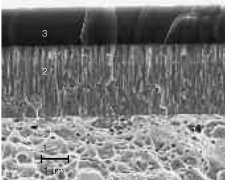
Typical structure of a multifunctional BALINIT® coating of the STAR series: 1 Base material (component) 2 CrN supporting layer 3 Tribologically effective carbon layer
