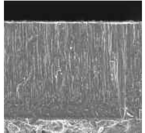
Coating structure of BALINIT® CNI
