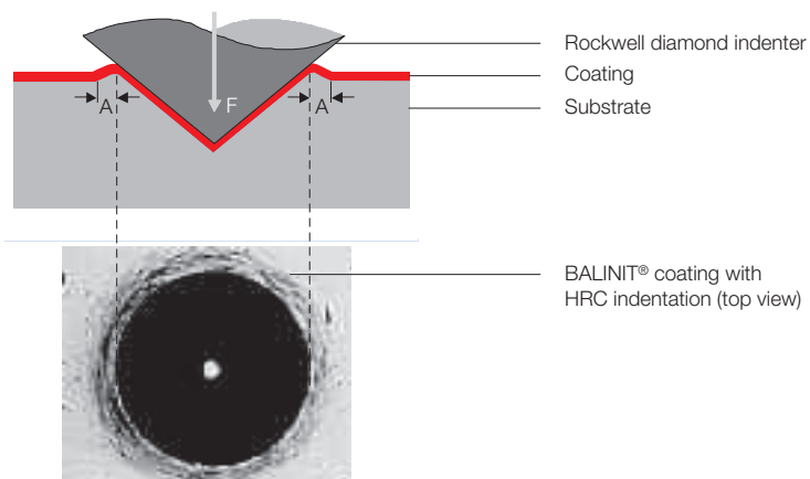
Use of Rockwell indentation to measure adhesion: Coating adhesion is determined by comparing the damage in region A of the Rockwell indentation to a series of standard images.
