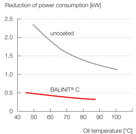
Reduction in truck rear-axle power consumption by BALINIT® coating
