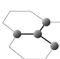
Graphite ( sp^2 )
