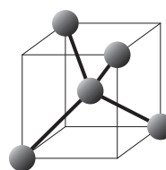
Diamond ( sp^3 )
