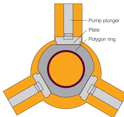
Schematic drawing of a diesel injection pump
