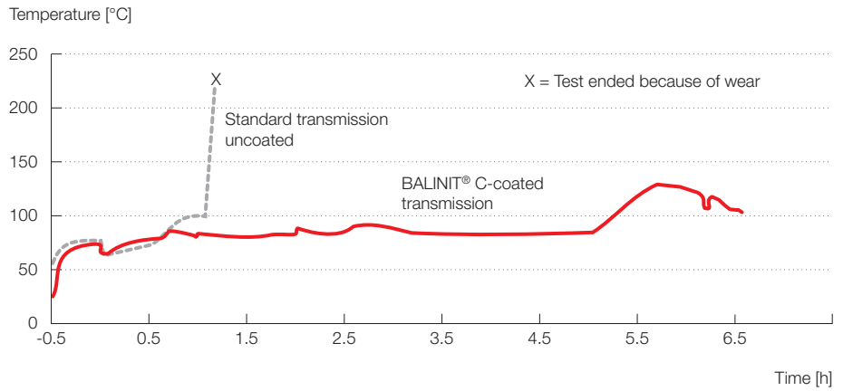
BALINIT® C-coated gears permit emergency operation for a considerably longer time after a loss of transmission fluid. Source: P. Maret and C. Varailhon / EUROCOPTER France
